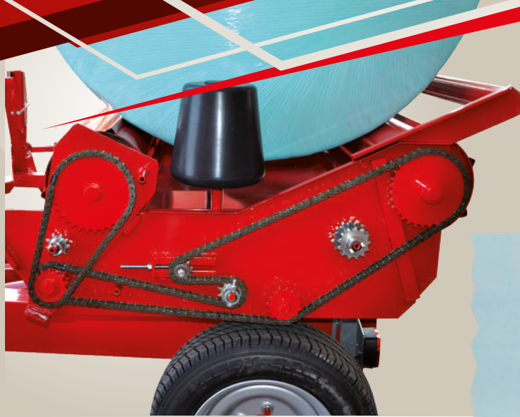
2 driving rollers, 1 of which is tilting, positioned on the platform, with 4 adjustable speeds, guarantee optimal work with all the dimensions of the bale.
