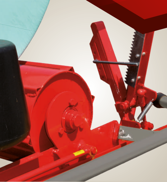
Automatic cutting of the film at the moment of tilting. (S and ST versions).
